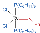
dichlorido(fenylmethylideen)bis(tricyclohexylfosfaan-κP)ruthenium, dichlorido(fenylmethaandiido)bis(tricyclohexylfosfaan-κP)ruthenium, of (benzylideen)dichloridobis(tricyclohexylfosfaan-κP)ruthenium
